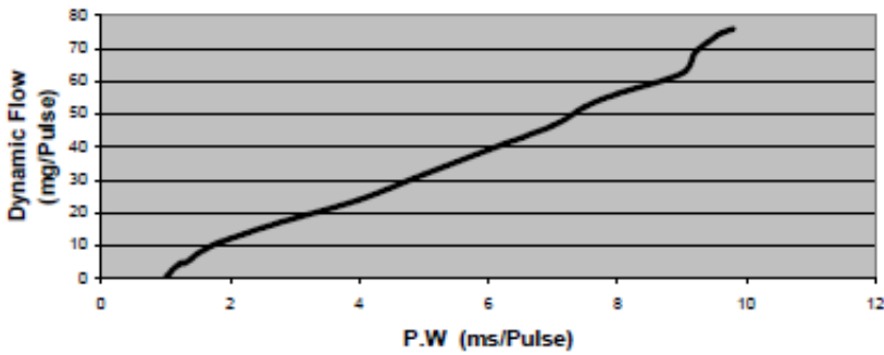
Min. Operating P.W Linearity Error, 0-10ms
